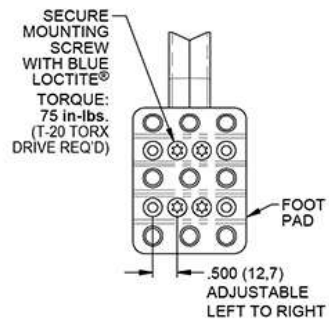
FOOT PAD DETAIL
